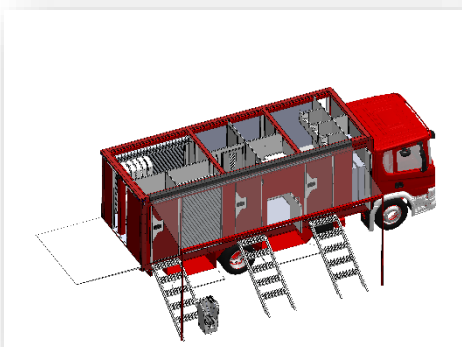
Vehicle body truck 16t
