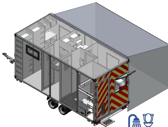
Vehicle body
